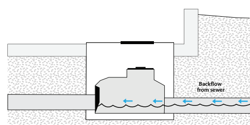
Install & Maintain a Backwater Valve
